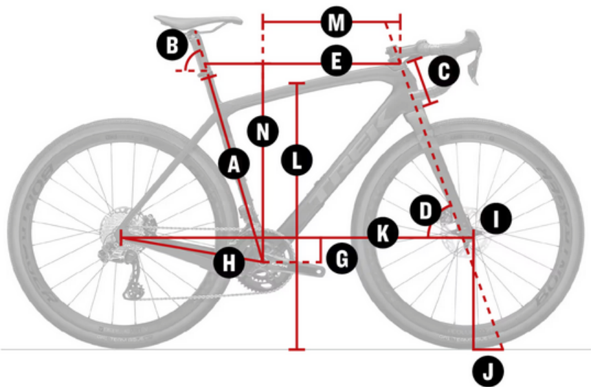
Geometry diagram labelling frame measurements A to N. Each label corresponds to a row in the geometry table below.
